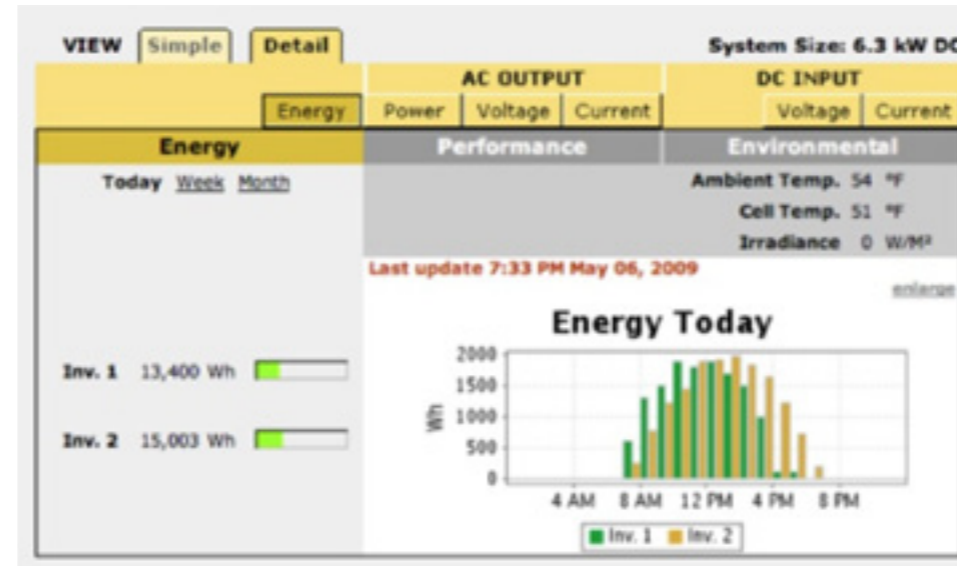
Green bars: Inverter one, Orange bars: Inverter two.
